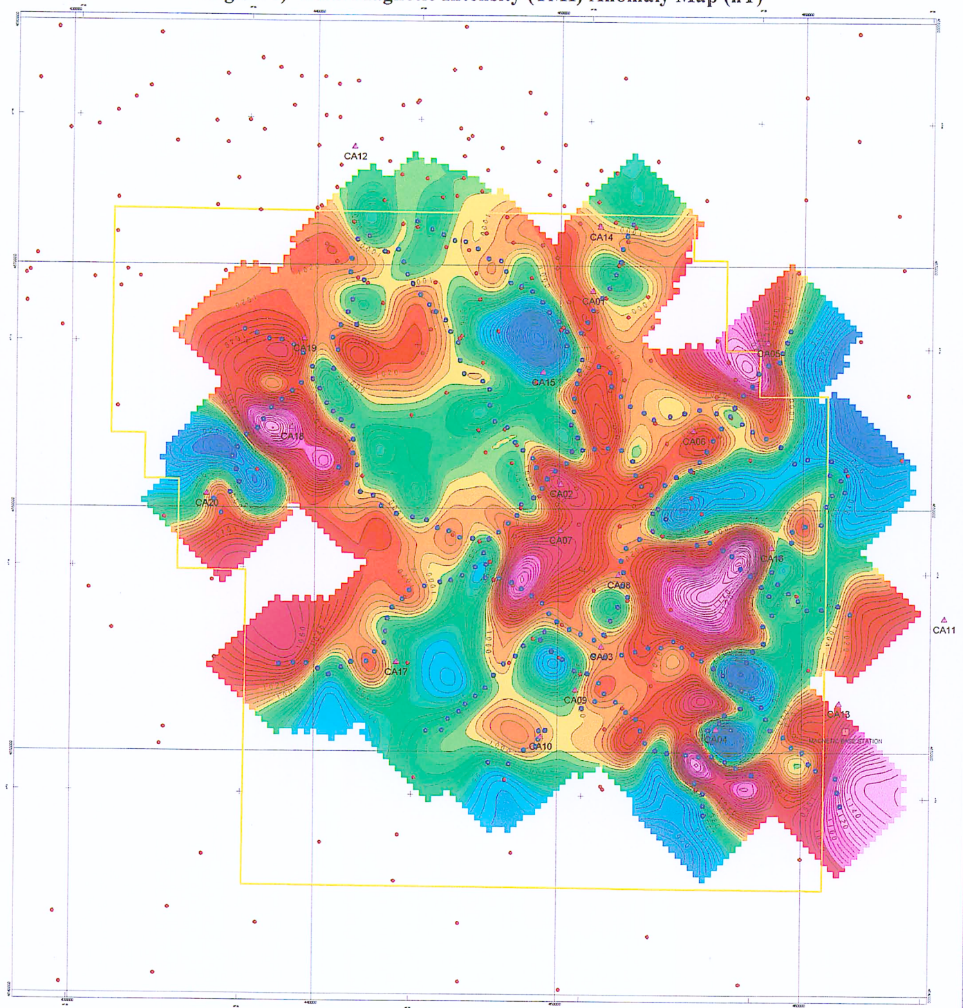
Figure 7) Total Magnetic Intensity (TMI) Anomaly Map (nT)
